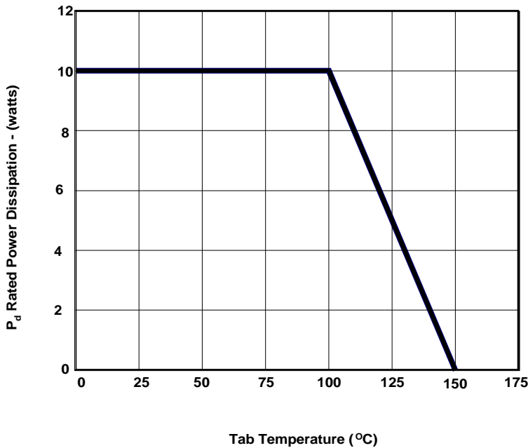
Figure 2 Power Derating Curve
